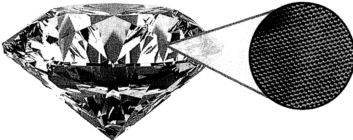
carbon atoms
