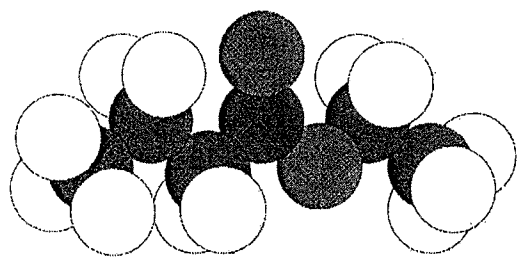
ethyl butyrate
