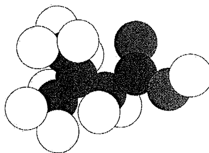
isovaleric acid
