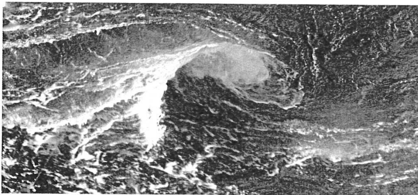
Ocean water is a mixture of compounds, including water (H 2 O), salt (NaCl), and others.
